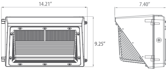
30W~70W OUTPUT
