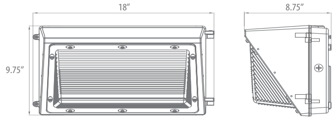
90W~140W OUTPUT
