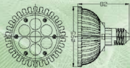
800 Lumens Turolux Vivid Solid State True Colour LED PAR30 with CryoDrive (TM) Inside 10.5W Warm White or Daylight White
