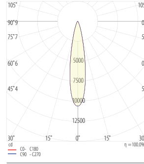
SP - 20° Spot, 4000K, 2100lm
