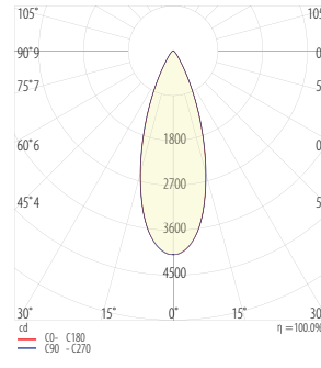
MF - 36° Medium Flood, 4000K, 2100lm
