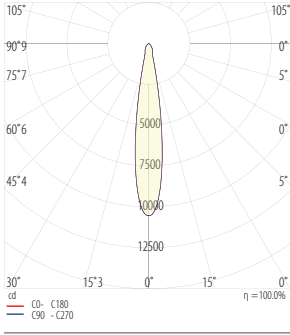
NS - 17° Narrow Spot, 4000K, 2100lm
