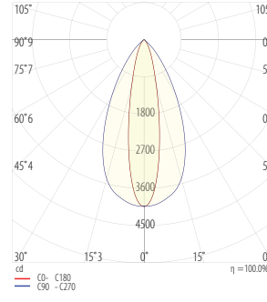
OV - 21 x 52° Oval Beam, 4000K, 2100lm
