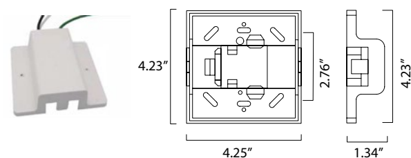
3-Wire Power Connector
